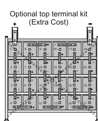
Front view 24 cells 2TLGM100 to 700 2 post cells
